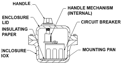
SECTIONED END VIEW OF ENCLOSURE WITH CIRCUIT BREAKER AND HANDLE MECHANISM INSTALLED
